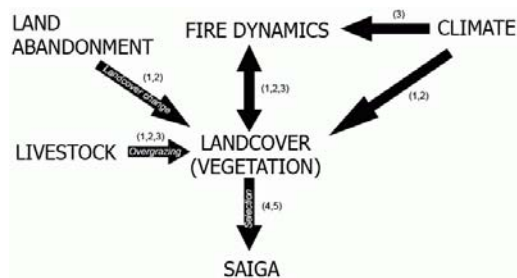
Figure 2. – Landcover change centered interactions; research questions numbers are given in parenthesis
