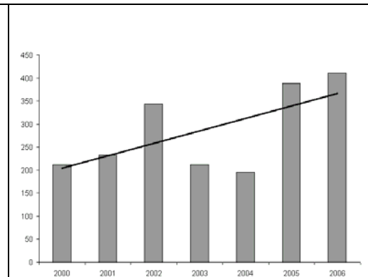
Figure 4. Recent changes in fire frequency for Republic of Kalmykia (MOD14 data, preliminary results)
