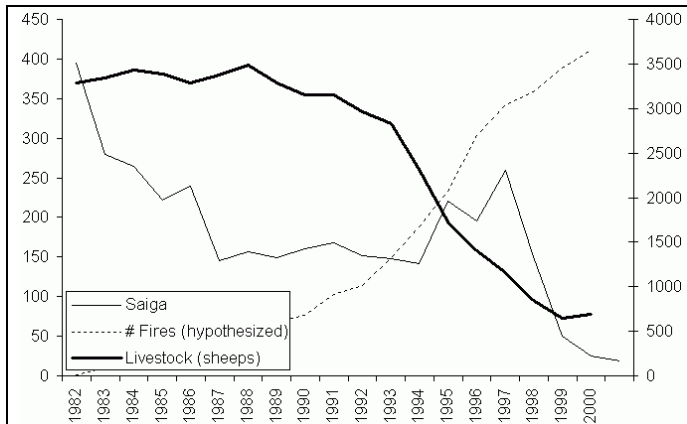
Figure 3. Change in hypothesized fire frequency, livestock and saiga populations in Kalmykia, right axis – livestock, left – saiga (Sokolov and Zhirnov 1998)
